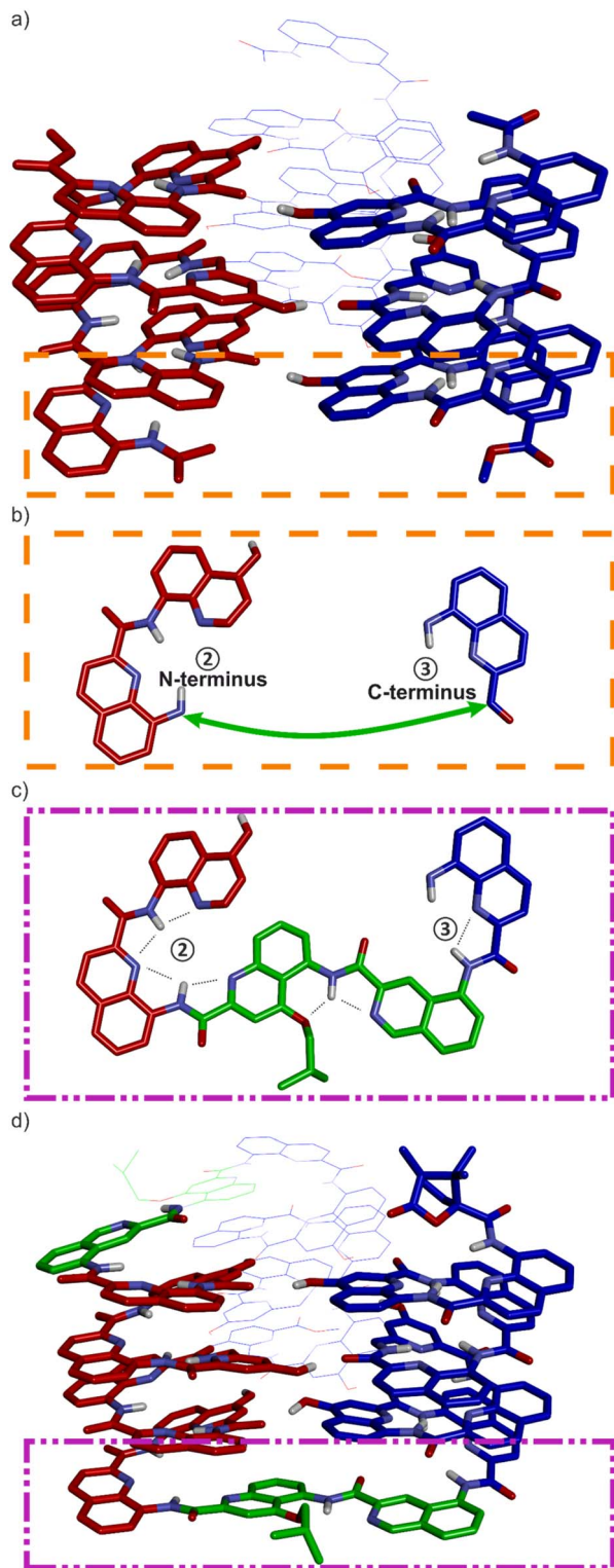
Fig. 3 (a) Energy-minimized model of a heterochiral (blue = P , red = M ) trimer of Ac-QXQYXQ-OMe. Helices in the front are in stick representation. The helix in the back is in line representation. (b) Top view of the terminal units within the orange dashed line box of (a). A green arrow shows where the turn unit should be placed. (c) Top view of the terminal units within the purple dashed line box of (d). (d) Energy-minimized model of 8b . Color coding is as in (a). The T6r turn is shown in green. In all structures, side chains on Q units have been omitted for clarity.
