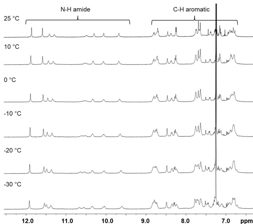
Figure S14. Part of the ^1\text{H} NMR spectra (400 MHz, \text{CDCl}_3/\text{CD}_3\text{OH} (95:5)) of 2^{\circ} \rightleftharpoons \text{D-fructose} (0.5 equiv.) at different temperatures, [2^{\circ}]_{\text{initial}} = 1.10 mM. The spectra depict chemical shifts variations of the amide protons and splitting of the hydrazodicarboxylate protons near 10.5 ppm. No indication of a slow exchange on the NMR time scale was observed even at low temperature.
