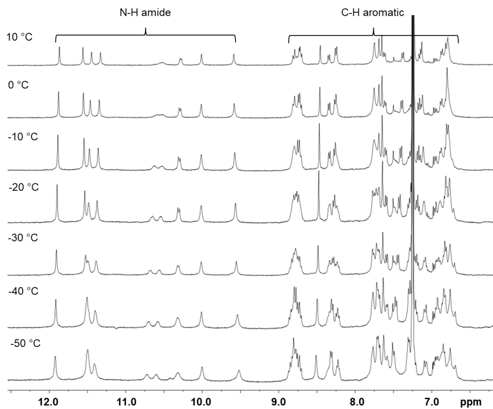
Figure S15. Partial 1 H NMR spectra (400 MHz, CDCl 3 /CD 3 OH (95:5)) of 2-D-fructose (1.0 equiv.) at different temperatures, [2 o ] initial = 0.98 mM. The spectra depict similar results as observed in Figure S16.
