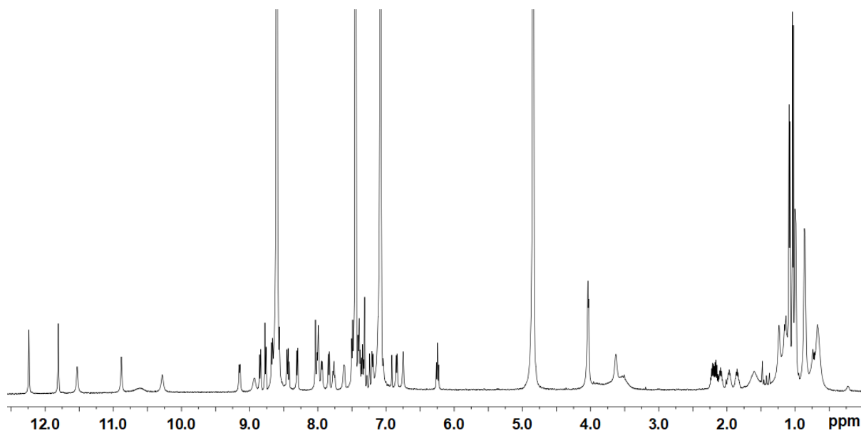
Figure S30. 1 H NMR spectra (500 MHz, 298K, Pyridine-d 5 ) of Capsule 1 .
