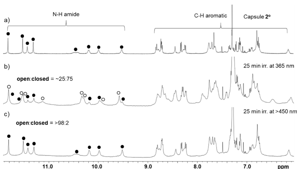
Figure S5. Partial 1 H NMR spectra (500 MHz, 298K, CDCl 3 /DMSO-d 6 (95:5)) at [2 o ] = 0.82 mM) of a) capsule 2 o (amide protons are depicted in black circles); b) after irradiation with 365 nm light (amide protons of the 2 c are depicted in open circles); c) after irradiation with >450 nm light. The presence of a single set of signals for both 2 o and 2 c is consistent with the presence of a single diastomeric conformer in which the two Q 3 PN 2 H segments either have same PP/MM or opposite PM handedness. The crystal structure of 2 o suggest that, for 2 o , this species is the PM conformer.
