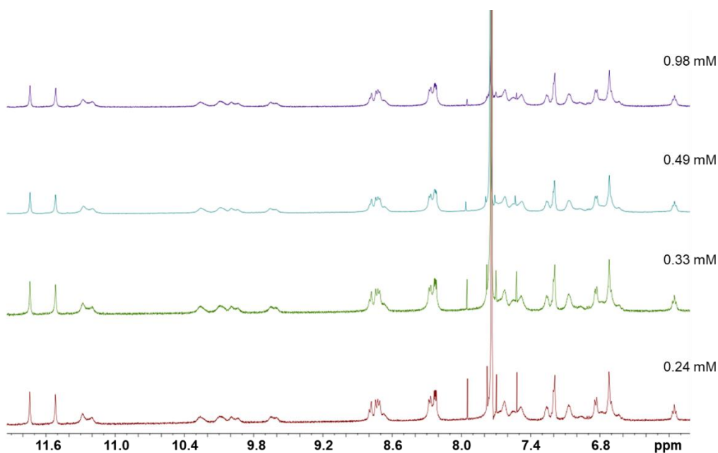
Figure S4. Partial ^1\text{H} NMR spectra (500 MHz, \text{CDCl}_3 , 298K) of capsule 2^{\circ} at different concentrations in 30/70 \text{DMSO-d}_6 : \text{CDCl}_3 vol/vol. The number of signals indicates a symmetrical structure on average, unlike the aggregated form observed in the solid state. The absence of chemical shift dependence of concentration suggests that the molecule is monomeric.
