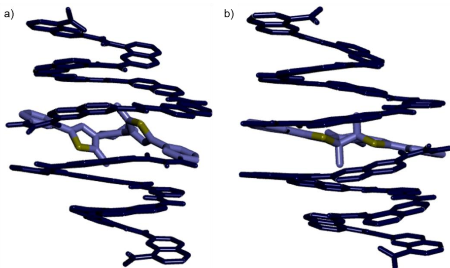
Figure S21. Energy minimized models (MacroModel, MMFFs force field) of a) 2^\circ and b) 2^c . Structural information alike to the capsule 1 were found.
