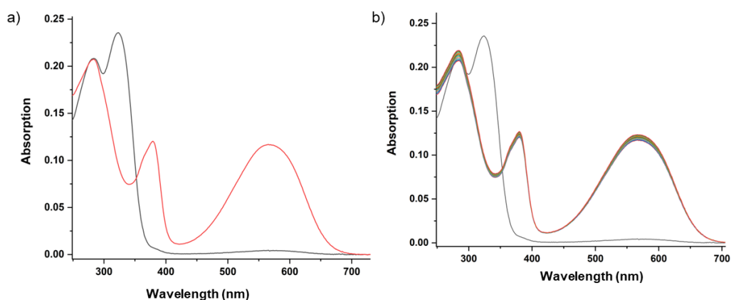
Figure S6. UV-Vis spectra (5% DMSO in chloroform at 1.2 \times 10^{-5} M) of a) light-induced switching (black and red traces are corresponding to 5^o and 5^c , respectively) and b) thermal stability studies over the period of 1h, suggesting that 5^c is thermally stable at room temperature over that period.
