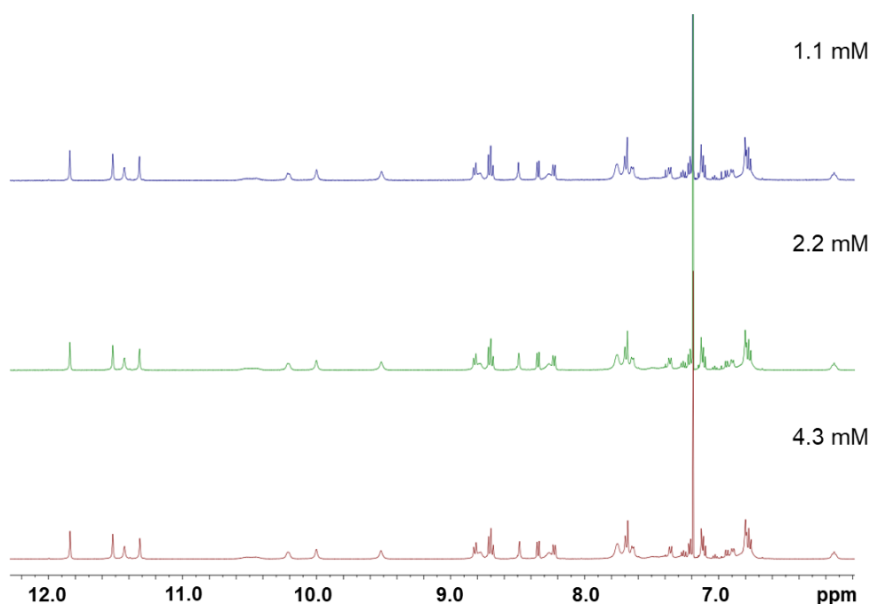
Figure S3. Partial ^1\text{H} NMR spectra (500 MHz, \text{CDCl}_3 , 298K) of capsule 2^{\circ} at different concentrations. The number of signals indicates a symmetrical structure on average, unlike the aggregated form observed in the solid state. The absence of chemical shift dependence of concentration suggests that the molecule is monomeric.
