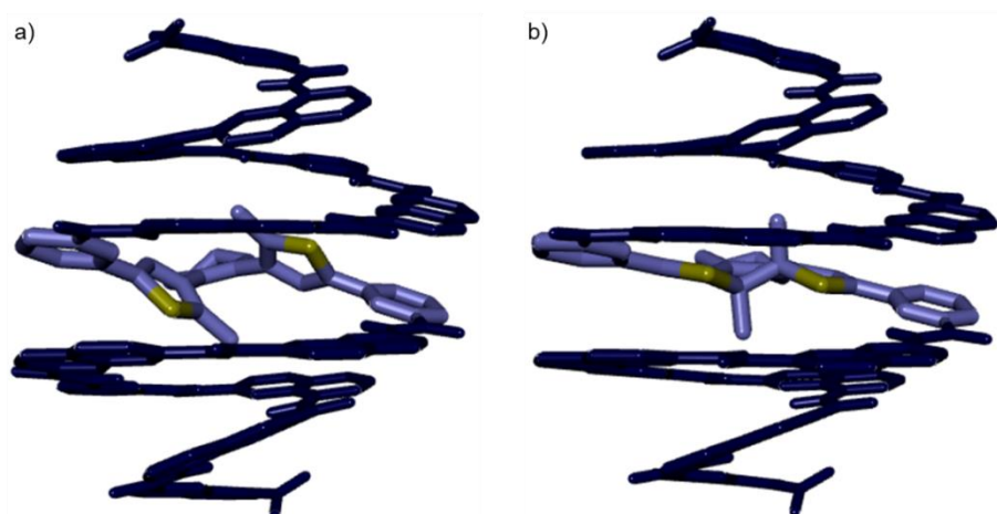
Figure S20. Energy minimized models (MacroModel, MMFFs force field) of a) 1^\circ and b) 1^c , suggesting helical conformation would not change upon ring closing. Additionally, the methyl groups protrude inside the cavity albeit at different orientations.
