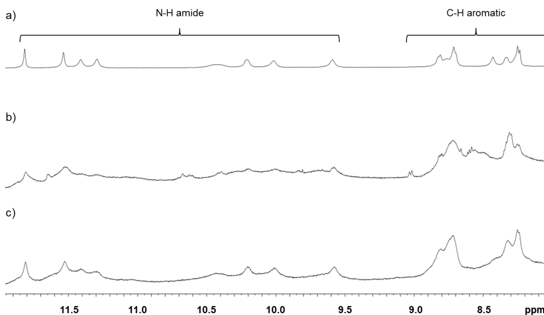
Figure S19. Part of the ^1\text{H} NMR spectra (500 MHz, 298K, in \text{CDCl}_3/\text{DMSO-d}_6 (95:5)) of a) 2^\circ\text{D} -fructose (2.25 equiv.); b) after irradiation with 365 nm light for 25 minutes; c) obtained after irradiation of the same solution with >450 nm light for 10 min at [2^\circ]_{\text{initial}} = 0.68 mM.
