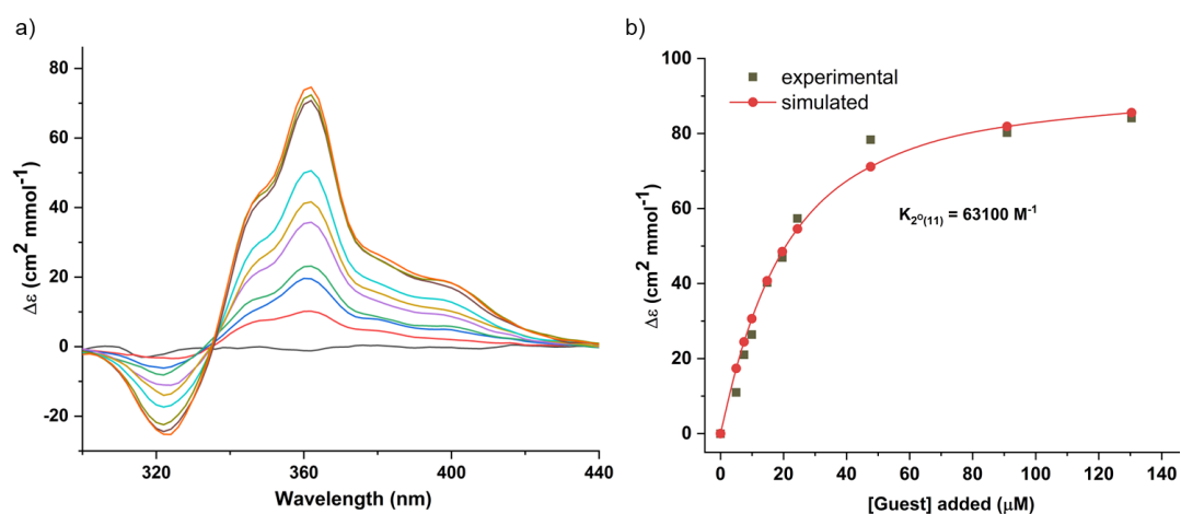
Figure S10. a) CD spectra (at 293K) for the binding of L-fructose by 2 o in \text{CHCl}_3/\text{DMSO} (95:5) at [\mathbf{2}^{\text{o}}]_{\text{initial}} = 10^{-5} \text{ M} . b) Curve fitting of binding isotherm using 1:1 binding model. This experiment mirrors that shown in Fig. 3a,b. The difference between binding constants reflect experimental variations.
