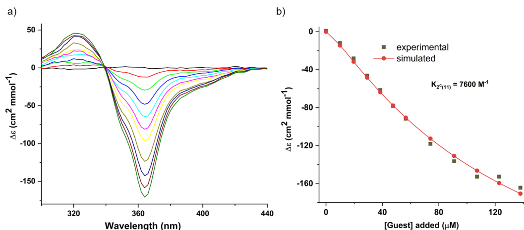
Figure S11. a) CD spectra recorded at 293K for the binding of L-fructose by 2^c in \text{CHCl}_3/\text{DMSO} (95:5) at [2^o]_{\text{initial}} = 10^{-5} M. b) Curve fitting of binding isotherm using 1:1 binding model taking into account the presence of 25% 2^o . This experiment mirrors that shown in Fig. 3c,d. The difference between binding constants reflect experimental variations.
