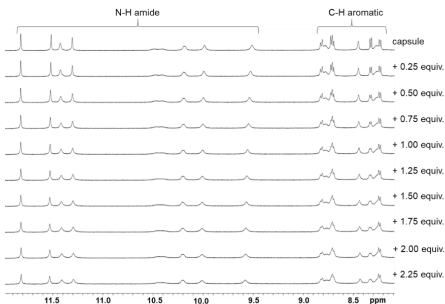
Figure S13. Part of the ^1\text{H} NMR spectra (500 MHz, 298K) of capsule 2^{\circ} in the presence of different amounts of L-fructose in \text{CDCl}_3/\text{DMSO-d}_6 (95:5) at [2^{\circ}]_{\text{initial}} = 0.82 mM. See Figure above for comments.
