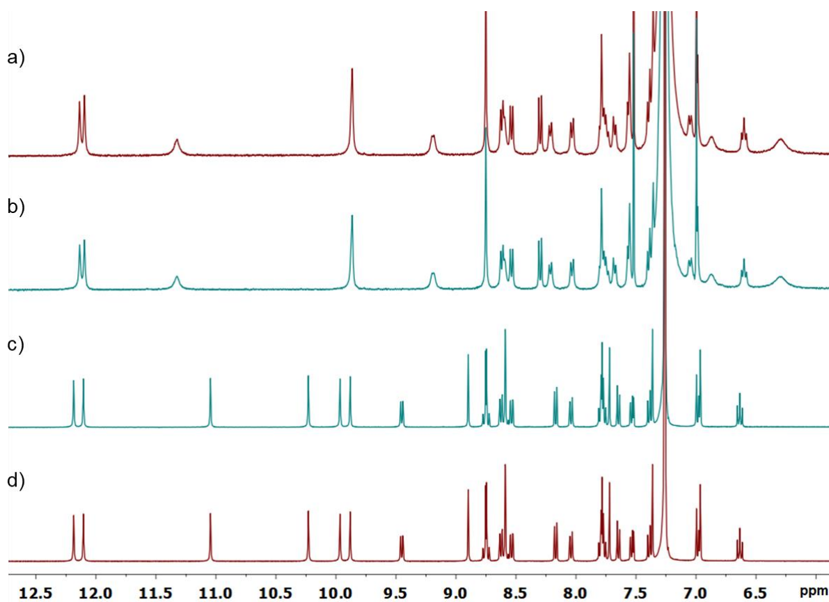
Figure S2. Partial ^1\text{H} NMR spectra (400 MHz, 298K) of free amine 7 (a) before and (b) after, and Boc- 7 (c) before and (d) after shining 365 nm light for 10 minutes in \text{CDCl}_3 .
