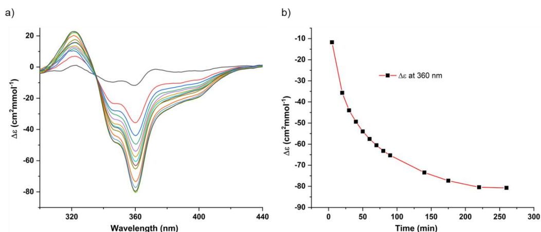
Figure S9. CD spectra (at 293K) for monitoring the kinetics of D-fructose binding by 2 o in \text{CHCl}_3/\text{DMSO} (95:5) at [\mathbf{2}^{\text{o}}] = 10^{-5} \text{ M} . The solution was treated with 25 equiv. of sugar and CD data were recorded over time. b) Plot of change in the \Delta\epsilon with respect to time. Note that this experiment does not tell about the inherent helix reversal rate of 2 o , but its reversal rate when saturated with fructose. One can envisage that fructose initially binds both P and M conformers and that binding slows down helix reversal.
