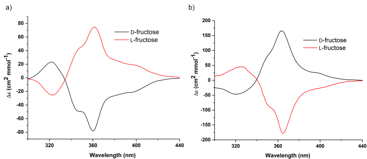
Figure S16. CD spectra (in 5% DMSO in chloroform at 10^{-5} M, 293K) in the presence of D- and L- fructose of a) 2^{\circ} and b) 2^{\text{c}} (PSS mixture obtained by irradiation prior to sugar addition).
