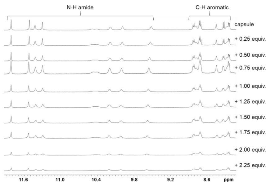
Figure S12. Part of the ^1\text{H} NMR spectra (500 MHz, 298K) of capsule 2^o in the presence of different amounts of D-fructose in \text{CDCl}_3/\text{DMSO}-d_6 (95:5) at [2^o]_{\text{initial}} = 0.86 mM. Continuous chemical shifts variations of amide protons are the result of fast exchange between 2^o and 2^o \rightleftharpoons \text{D-fructose} on the NMR times scale. The NMR lines broaden because fructose exists in different \alpha/\beta and pyranose/furanose configurations which each may engage in more than one binding complex geometry. The broadening of the lines is probably the reason why different sets of signals are not observed for MM- 2 \subset fructose and PM- 2 \subset fructose, which must equilibrate slowly on the NMR time scale.
