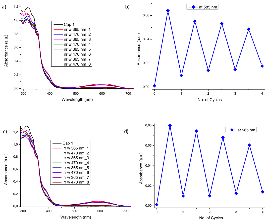
Figure S7. a) UV-Vis spectra of capsule 1 depicting reversible switching upon irradiation with \lambda = 365 nm and \lambda > 450 nm light in chloroform/DMSO (95:5) at [1^o] = 10^{-5} M. b) Change in absorption spectra monitored at 585 nm upon reversible light irradiation, depicting the reversibility of switching and suggesting some fatigue upon prolonged exposure to light. c) and
