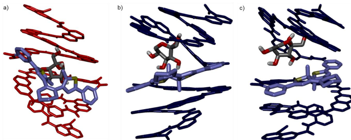
Figure S22. Energy minimized models (MacroModel, MMFFs force field) of a) 2^{\circ}\supset\alpha -D-fructopyranose (the capsule completely secludes the guest) and b-c) different views of 2^{\circ}\supset\alpha -D-fructopyranose (the guest moves to one hemi-capsule in order to avoid interference from the methyl group).
