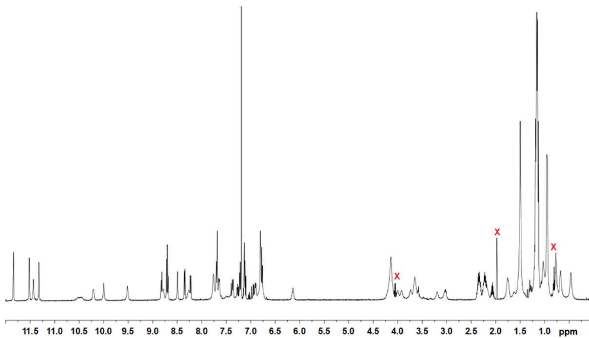
Figure S31. 1 H NMR spectra (500 MHz, 298K, CDCl 3 ) of capsule 2 . Signals assigned with red crosses are corresponding to ethyl acetate.
