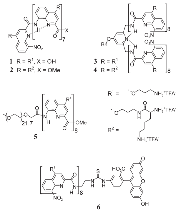
Figure 2. Water-soluble helical aromatic amide foldamers. Bn = benzyl, TFA = trifluoroacetate.
