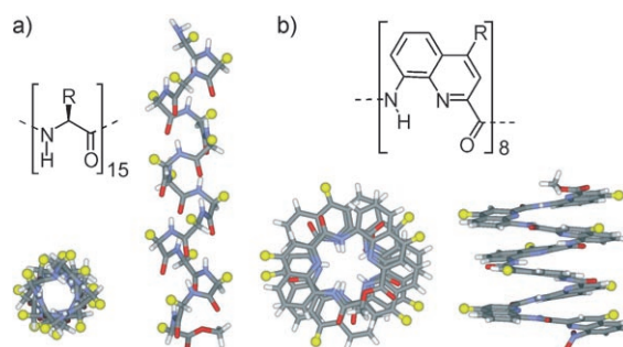
Figure 1. Top view and side views of fragments shown at the same scale of crystal structures of: a) a peptide \alpha helix and b) a helix of an aromatic oligoamide foldamer. Side chains (R) are shown as yellow spheres. These structures illustrate the striking differences between the two motifs in terms of side-chain density, diameter, aspect ratio (at comparable molecular weight), helical pitch, and overall chemical composition.
