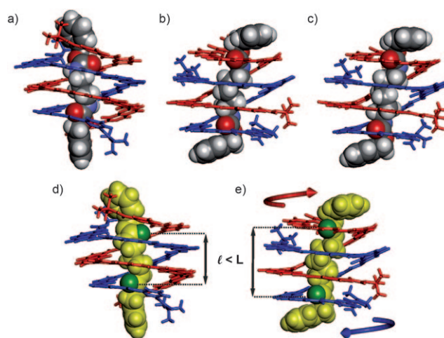
Figure 3. Solid-state structures of a) (\mathbf{1})_2 \supset \mathbf{2b} , b) (\mathbf{1})_2 \supset \mathbf{2d} , and c) (\mathbf{1})_2 \supset \mathbf{2e} . The antiparallel strands of (\mathbf{1})_2 are shown in red and blue (tube representation). Rodlike guests are shown in CPK (C gray, H white, O red, N light blue). Illustrations of the screw motion are shown in d) (\mathbf{1})_2 \supset \mathbf{2b} ; and e) (\mathbf{1})_2 \supset \mathbf{2d} . Rods are in yellow CPK representations. The carbonyl oxygen atoms of the carbamate groups are shown in green. L and l represent the distance between the two pyridine clefts in each complex (\mathbf{1})_2 \supset \mathbf{2b} and (\mathbf{1})_2 \supset \mathbf{2d} , and are equal to 6.8 Å and 9.0 Å, respectively. The red and blue arrows illustrate the screw-motion mechanism between complex (\mathbf{1})_2 \supset \mathbf{2b} and (\mathbf{1})_2 \supset \mathbf{2d} . Isobutyl side chains and included solvent molecules have been omitted for clarity.
