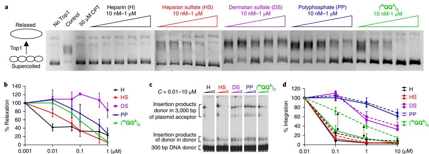
Fig. 4 | Inhibition of Top1 and HIV-IN by polyanions. a , Inhibition of Top1-mediated relaxation of supercoiled circular DNA by various polyanions and (^m\text{QQ}^4)_8 assessed by gel electrophoresis. The control lane shows full Top1 activity. Camptothecin (CPT) is a classical Top1 inhibitor. b , Quantitation of Top1 inhibition expressed as a percentage of relaxation as compared to the control. c , Inhibition of in vitro HIV-IN integration (200 nM of IN) of a radio-labelled 246 bp viral DNA donor into a 2,700 bp pZeo plasmid acceptor assessed by agarose gel electrophoresis using the same polyanions. d , Quantitation of the inhibition of wild-type HIV-IN (solid lines) and K236A HIV-IN (dashed lines) by polyanions and (^m\text{QQ}^4)_8 , expressed as a percentage of integration relative to a control in the absence of inhibitors. Double-headed arrows indicate the selectivity of (^m\text{QQ}^4)_8 . In a and c , quantitation was obtained by analysis of the gels using ImageJ software. Results are the means of triplicate experiments \pm standard deviation.
